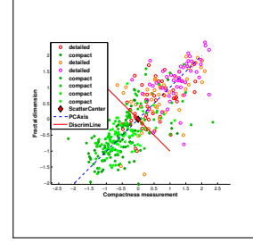
Fig. 1: The scatter plot of FD and CM .
