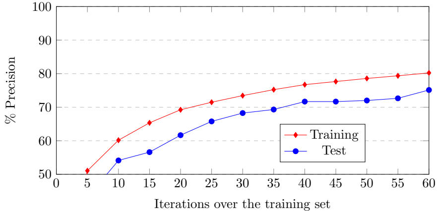
Figure 7: Training and test precision achieved by Nurbsnet after 60 training iterations using the ModelNet40 dataset with 2 internal Nurbs
