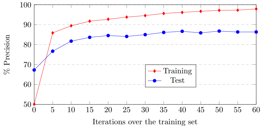
Figure 5: Training and test precision achieved by Nurb-net after 60 training iterations using the ModelNet10 dataset with 2 internal Nurbs
