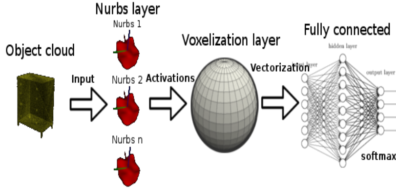
Figure 3: End-to-end network scheme of our proposal
