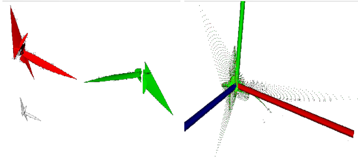
Figure 2: Red, green and grey nurbs surfaces in the left have the same shape but different scale, rotation and translation. They are represented in the right with the same sample points in euclidean space after the use of the techniques explained in Section 3.1.2
