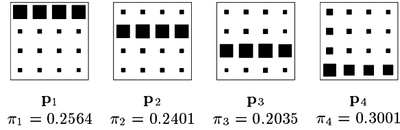
Figure 2: Parameters of a mixture of M = 4 16-variate Bernoulli distributions estimated by maximum likelihood from the sample. Observe that \mathbf{p}_1 , \mathbf{p}_2 , \mathbf{p}_3 and \mathbf{p}_4 coincide very closely with \mathbf{p}_1^o , \mathbf{p}_2^o , \mathbf{p}_3^o and \frac{2}{3}\mathbf{p}_4^o + \frac{1}{3}\mathbf{p}_5^o , respectively.
