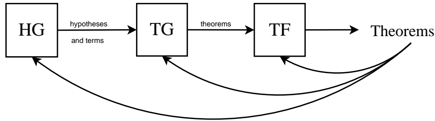
Fig. 1. Component Diagram
