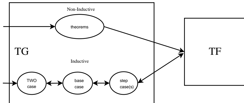
Fig. 3. Theorem Generator
