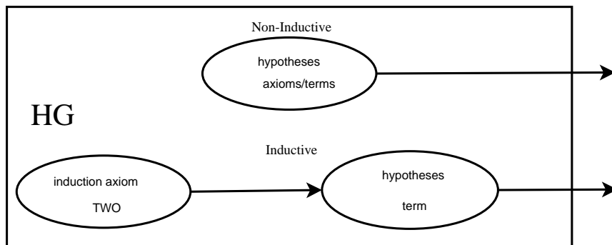
Fig. 2. Hypothesis/Term Generator
