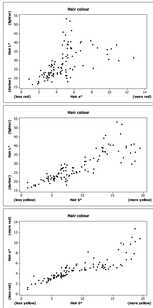
Figure 1 L^* (dark/light) a^* (red) b^* (yellow) values (hair colour) measured by tristimulus colorimetry in 107 Scots from Edinburgh. Each individual is plotted as L^* vs a^* (top), L^* vs b^* (middle) and a^* vs b^* (bottom).
